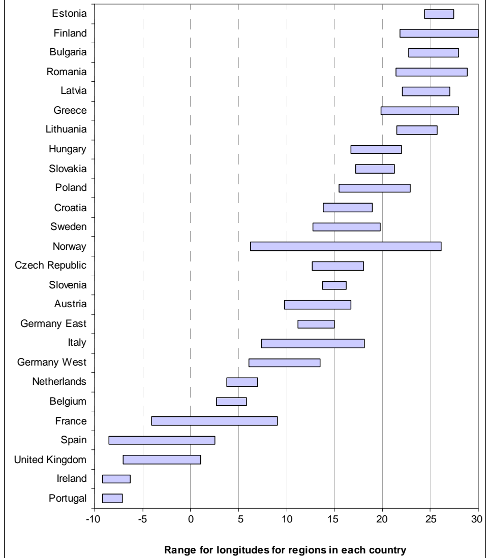
Figure A1: Longitudes of European countries
