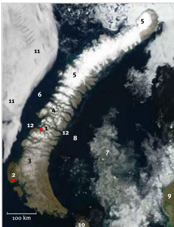
Fig 2. Satellite summer image of Novaya Zemlya area
